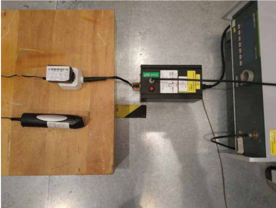
Injected currents (RF continues conducted)
