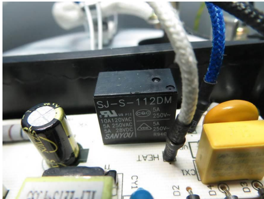
Relay for RCD-YY
