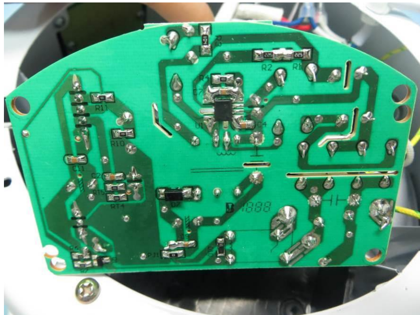
Power PCB (Back) for RCD-YY
