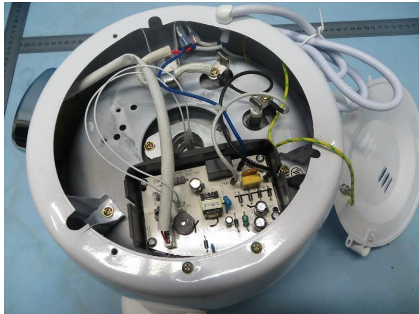
Inner view for RCD-YY
