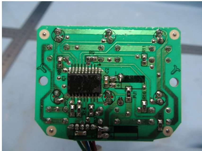
Control PCB (Back) for RCD-YY
