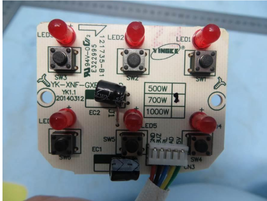
Control PCB (Front) for RCD-YY
