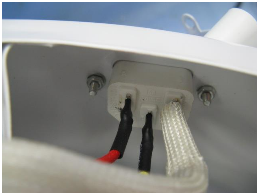
Fig. 18: Appliance inlet
