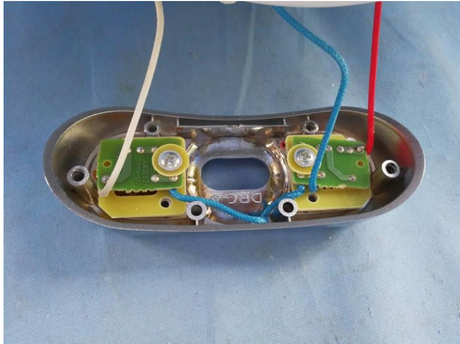
Inner view for DRC-5
