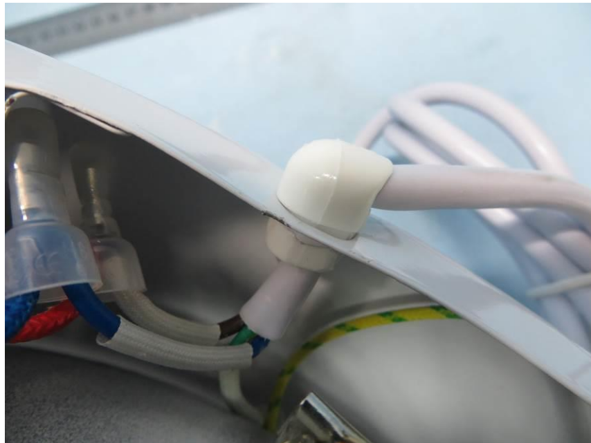
Cord anchorage for RCD-YY
