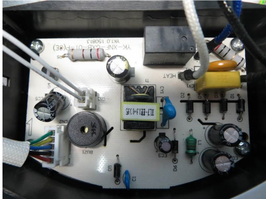
Power PCB (Front) for RCD-YY
