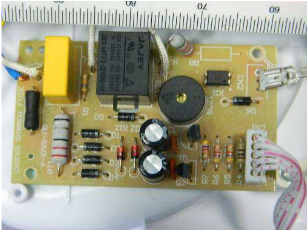
PCB view of KL-916C and KL-916D
