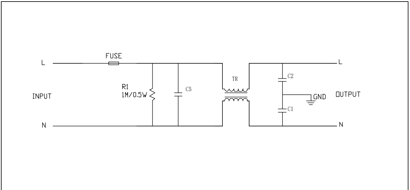
Circuit diagram Noise filter PCB FN14-1K00, FN14-1K06
