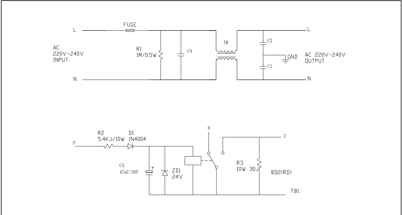
Circuit diagram Noise filter PCB FN14-1K00, FN14-1K06
