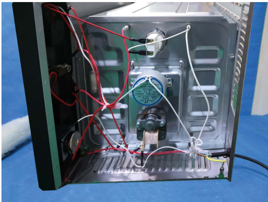
Internal view (after removed thermal insulation material )
