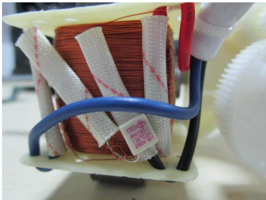
Thermal-link view
