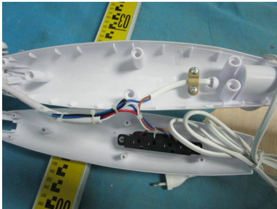
Internal view of YH-40A-y
