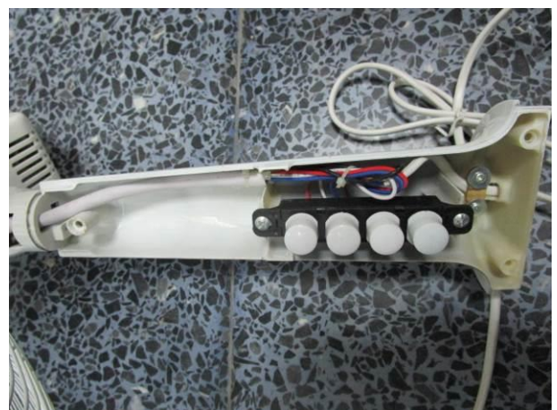
Internal view
