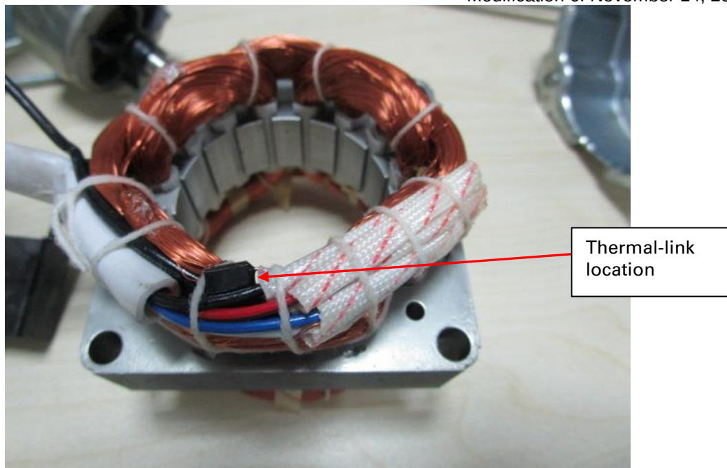
Internal view
