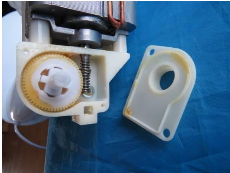
Rotor box view
