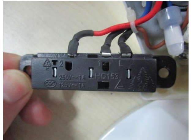
Speed switch view
