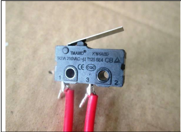
55. Interlock switch
