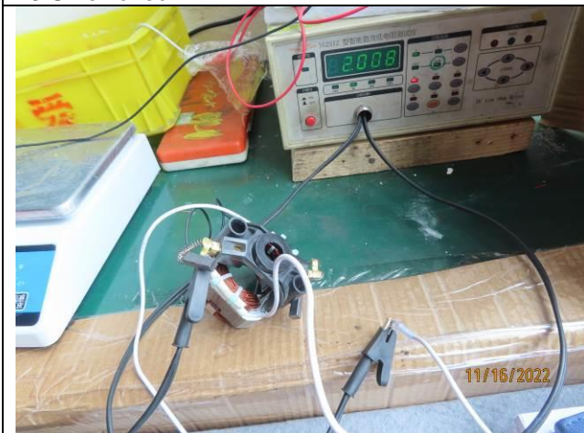
75. Motor resistance check
