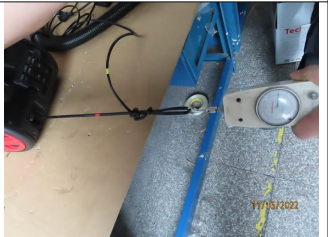
70. Strain relief test
