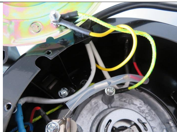
20. Earth connection
