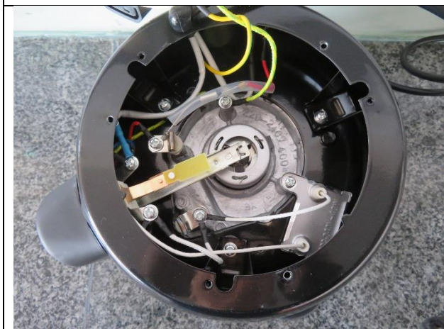
21. Internal view
