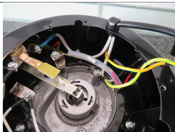
22. Internal view
