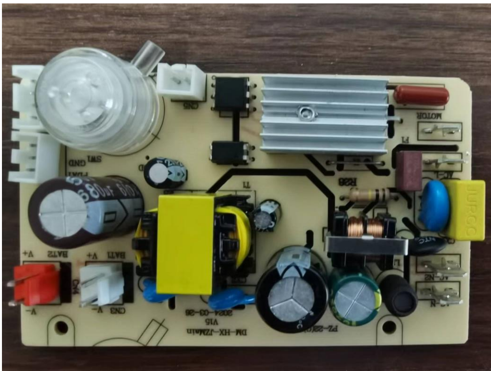
Alternative PCB
