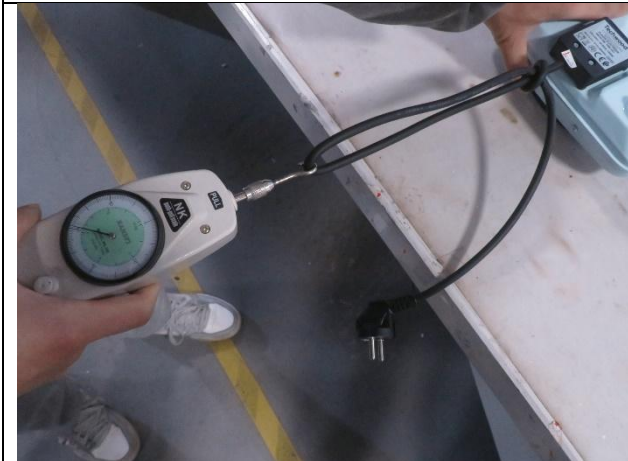
113. Strain relief test
