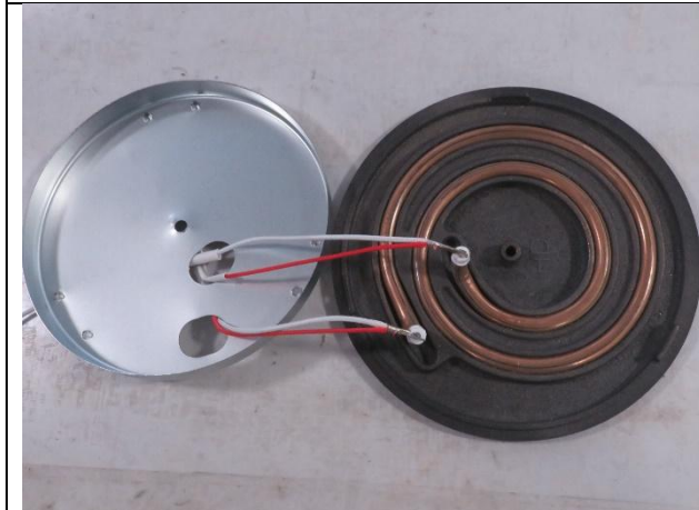
107. Heating element
