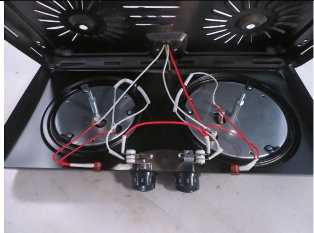
98. Product inner view
