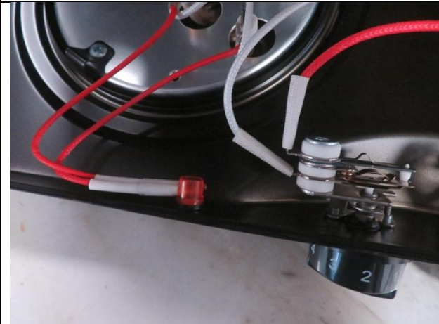
101. Product inner view
