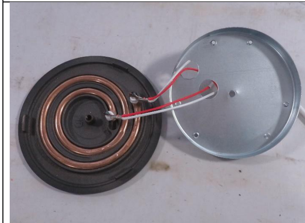
105. Heating element
