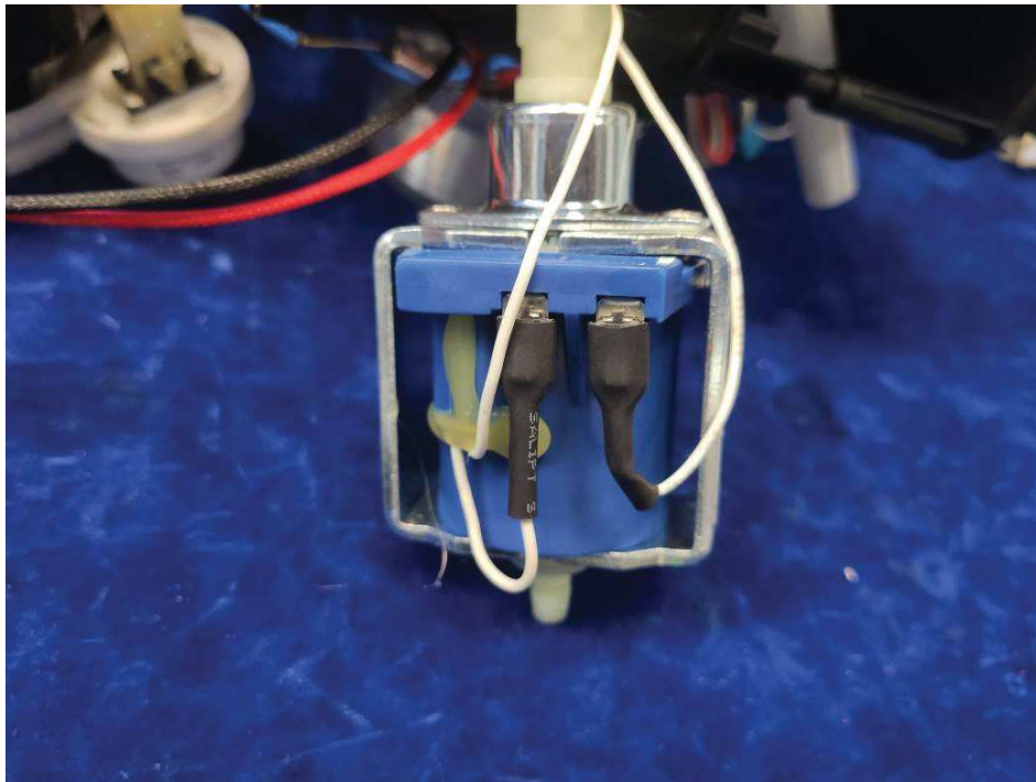
Pump
