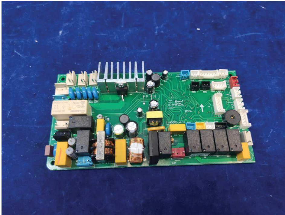
Main PCB
