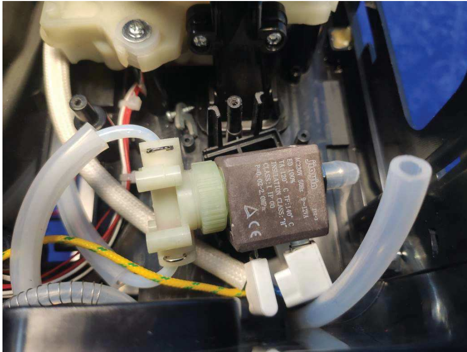
Solenoid valve
