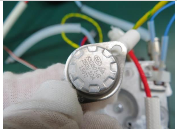
194. Thermostat
