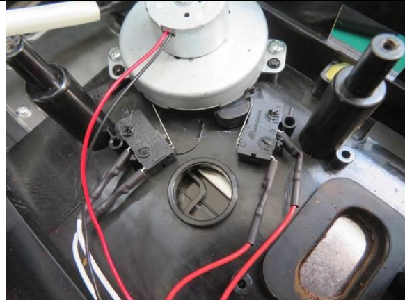
147. Internal view
