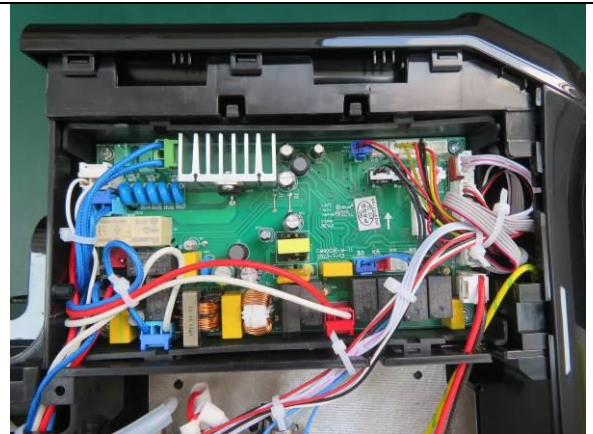
136. Internal view
