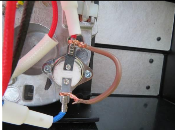
231. Thermal fuse function check
