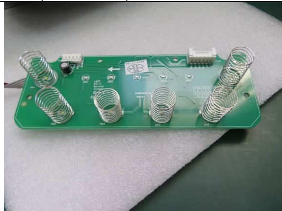
151. Control PCB
