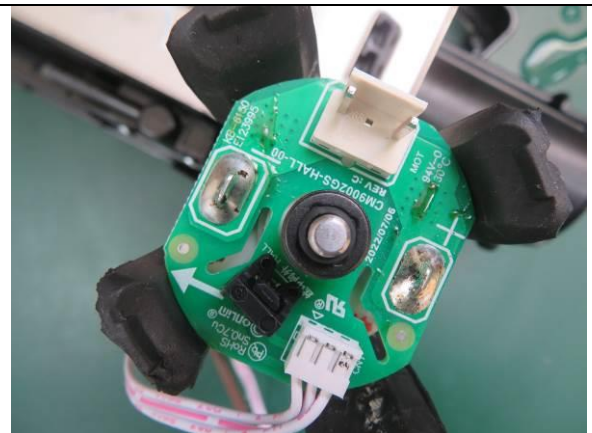
186. PCB on brewing motor
