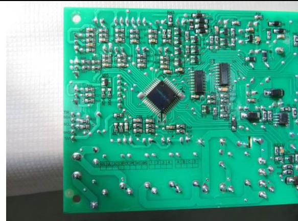
159. Main PCB
