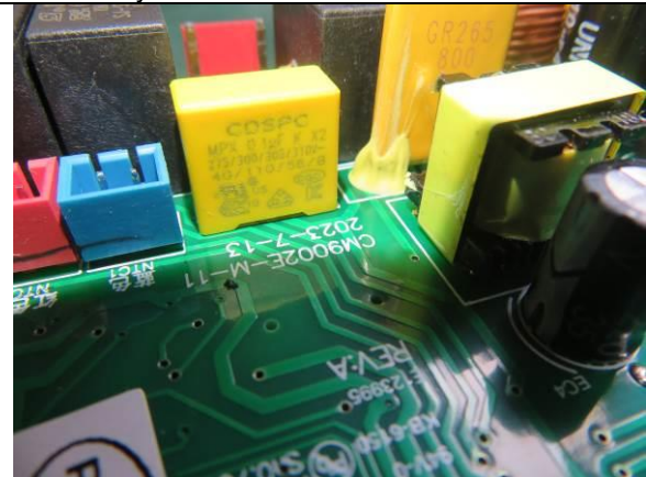
165. X capacitor
