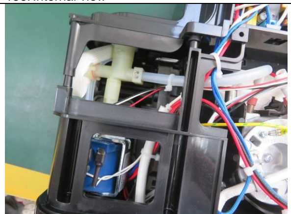
138. Internal view
