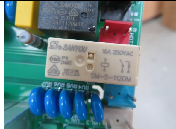
163. Relay
