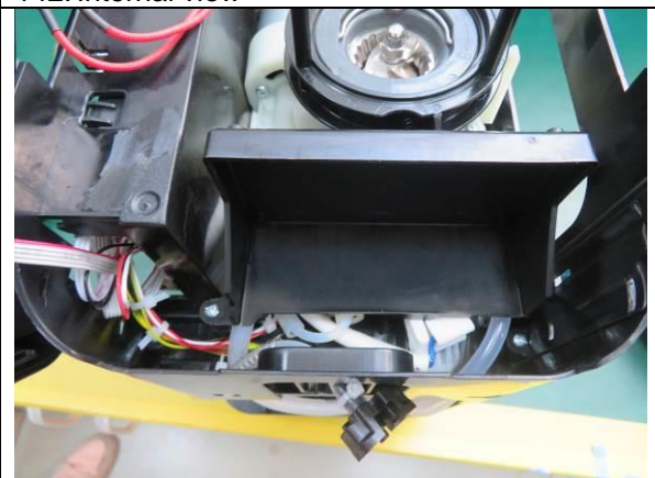
144. Internal view
