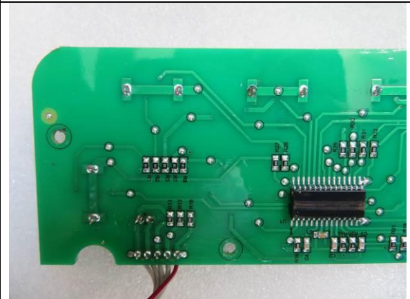
154. Control PCB
