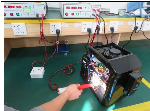
207. Earth continuity test
