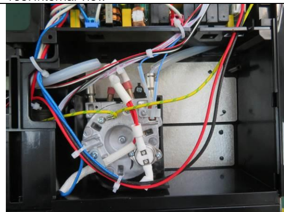
137. Internal view
