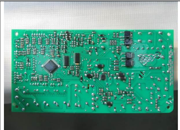
158. Main PCB
