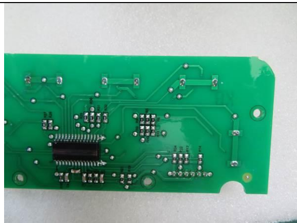
155. Control PCB
