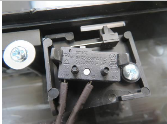
149. Internal view
