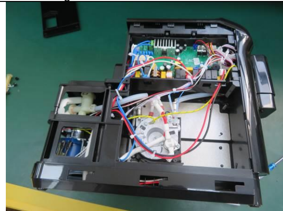
135. Internal view
