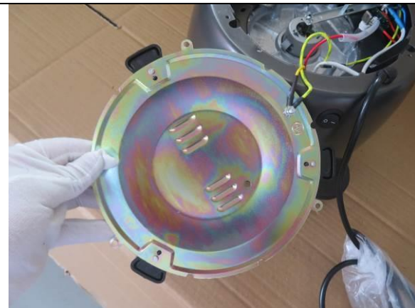
269. Internal view
