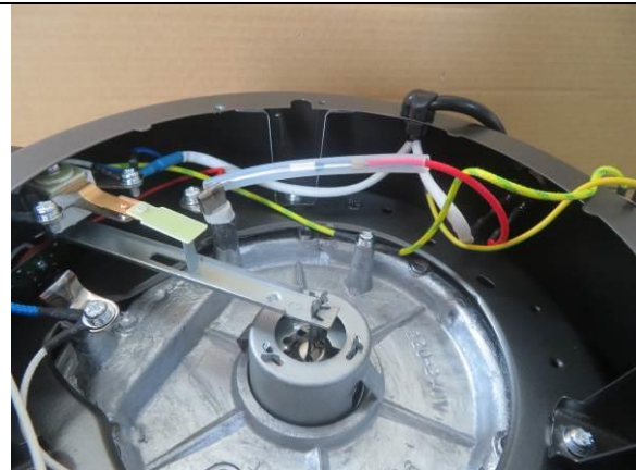
274. Internal view
