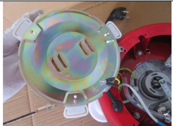
74. Internal view
