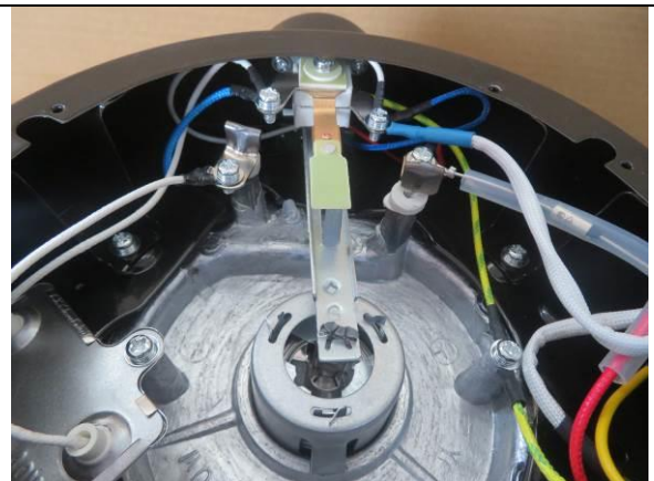
168. Internal view
