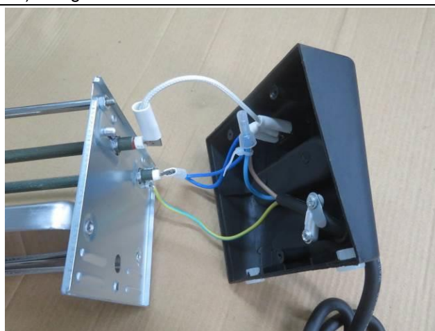
58) Internal workmanship
