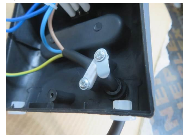
59) Internal workmanship
