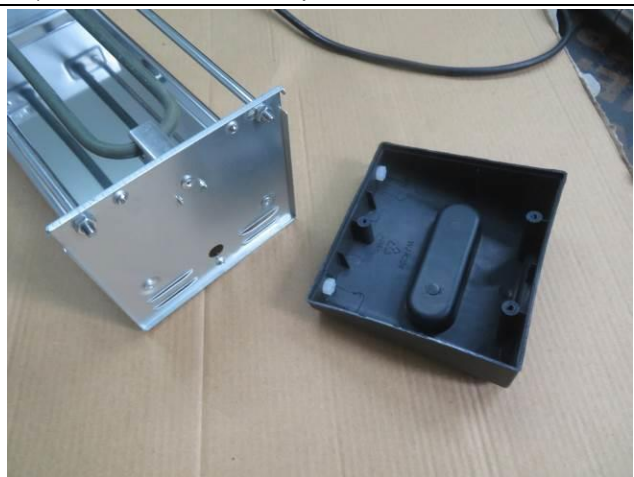
64) Internal workmanship
