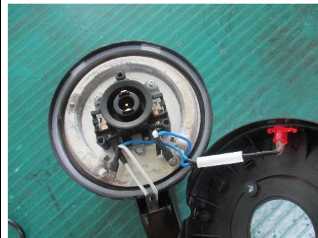
77. Internal view
